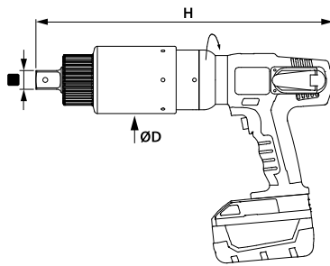
LDA series – straight version
